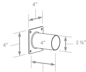
Wall Mount Bracket LEDMPALPRO-WMB
