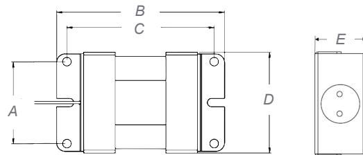
Battery Bracket
